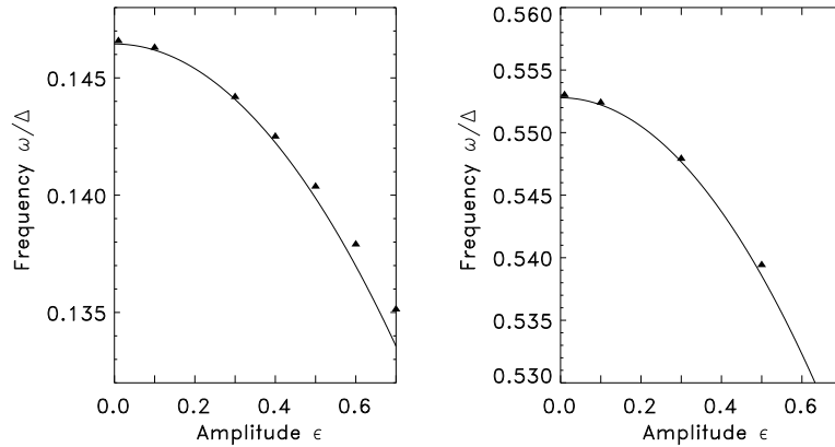
Figure 3. Non-dimensional wave frequency against wave amplitude \epsilon . Model calculations (triangles) are compared with weakly nonlinear predictions from (37), (curves). The left panel shows waves with kL_R = 1 , with numerical experiments for \epsilon = 0.01, 0.1, 0.3, 0.4, 0.5, 0.6 and 0.7 and in the right panel kL_R = 2 , \epsilon = 0.01, 0.1, 0.3 , and 0.5 .
