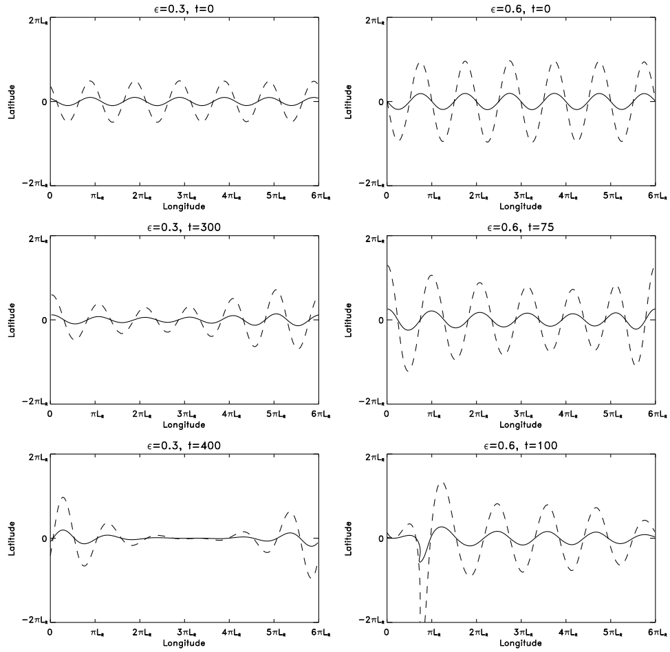
Figure 5. Snapshots of the contour evolution in the \epsilon = 0.3 experiment (left panels) and the \epsilon = 0.6 experiment (right panels). In the \epsilon = 0.3 case the snapshots are for times t = 0, 300 and 400 \times 2\pi\Delta^{-1} , and for \epsilon = 0.6 they are for t = 0, 75 and 100 \times 2\pi\Delta^{-1} . The dashed curves show the same waves plotted with 5 \times their actual amplitude for clarity.
