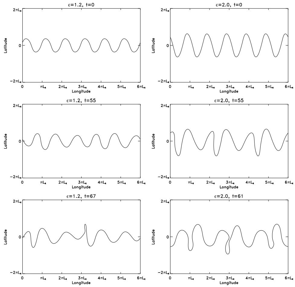
Figure 6. Snapshots of the contour evolution for \epsilon = 1.2 (left) and \epsilon = 2.0 (right) experiments. Time units are again 2\pi\Delta^{-1} .
