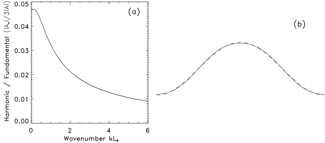
Figure 2. (a) The third harmonic amplitude divided by fundamental amplitude for the weakly nonlinear Rossby waves as a function of wavenumber kL_R . (b) Showing the leading order correction to the shape of the potential vorticity contour (solid line) \eta_0 + \epsilon^2 \eta_2 predicted by equations (14), (26) and (36) for kL_R = 1 (with \epsilon|A|=1 ). The dashed line shows the sinusoidal wave \eta_0 .
