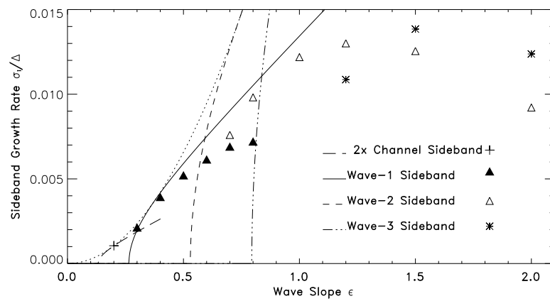
Figure 4. Sideband growth rate against wave amplitude \epsilon . Model calculations (triangles) are compared with weakly nonlinear predictions from (34). In the calculations the initial wavelength kL_R = 1 and the domain is periodic with length scale L_x = 12\pi k^{-1} . The predicted growth rates of wave-1, wave-2 and wave-3 sideband modulations (see text) are given by the solid, dashed and dot-dashed curves respectively. The curve with long dashes shows the predicted wave-1 sideband growth rates in a domain with double the size, and the dotted curve show the predicted sideband growth rates for an infinite domain. The solid triangles show the wave-1 sideband growth rates for the numerical experiments, and the unfilled triangles shows the wave-2 sideband growth rate. For \epsilon = 0.7 and higher the wave-2 sideband growth dominates.
